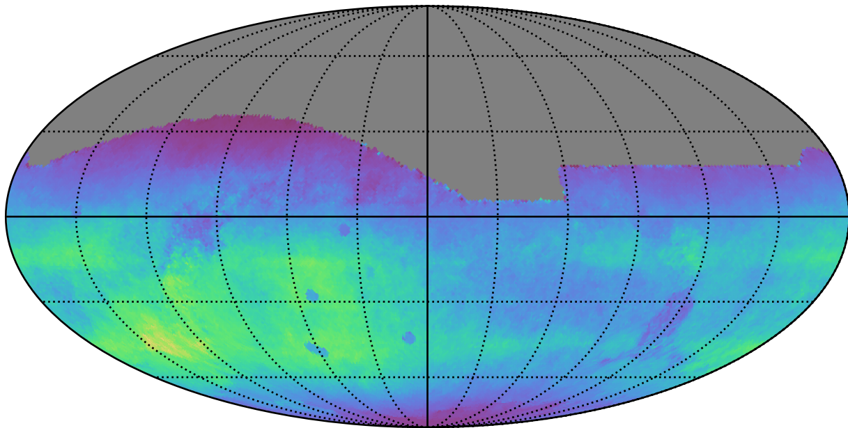
extra_ss_neo3_v3.4_10yrs All sky r band: Normalized Teff
