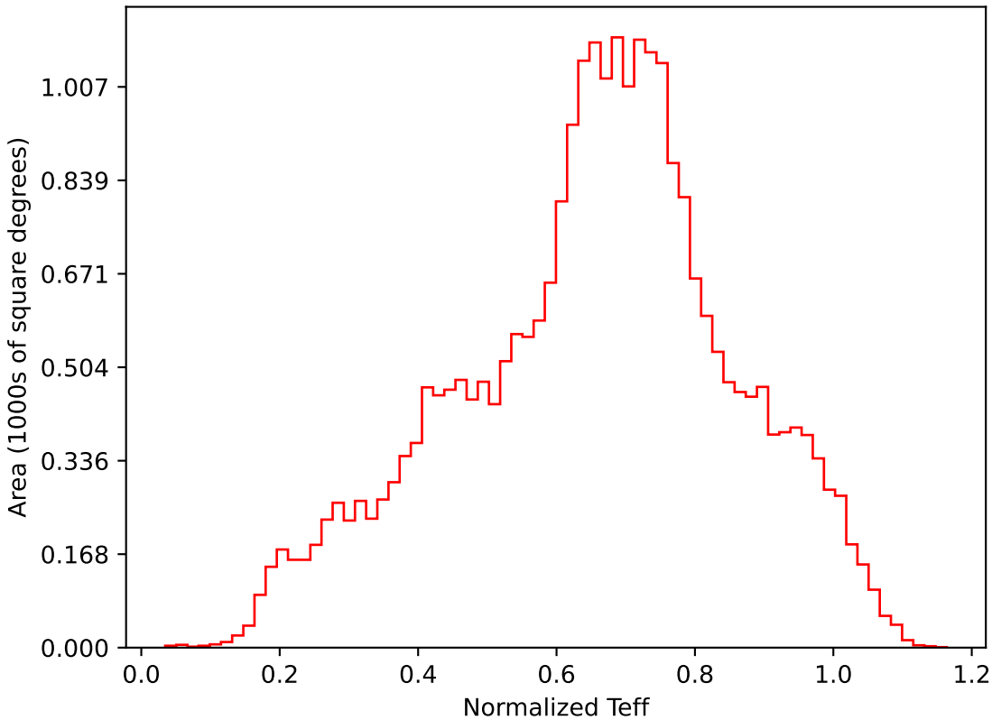
extra_ss_neo3_v3.4_10yrs All sky i band: Normalized Teff
