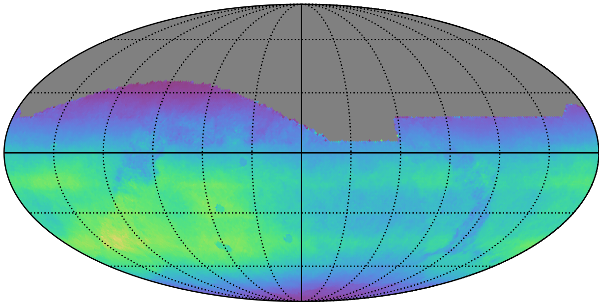
extra_ss_neo3_v3.4_10yrs All sky all bands: Normalized Teff
