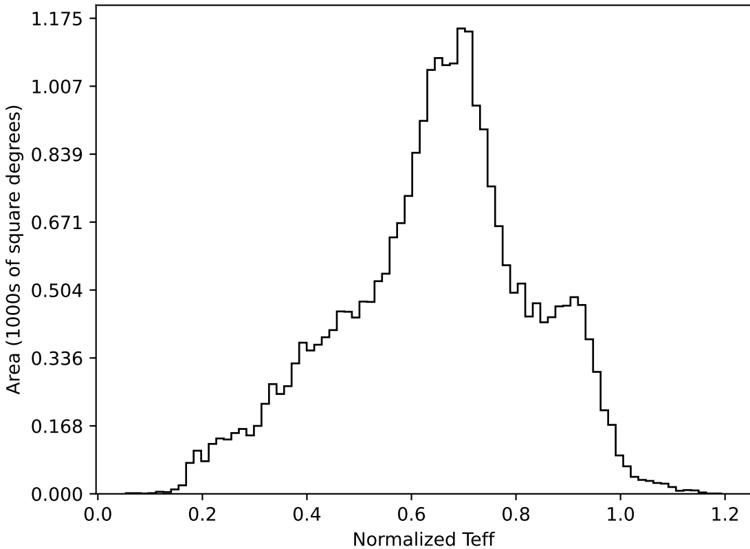
extra_ss_neo3_v3.4_10yrs All sky all bands: Normalized Teff
