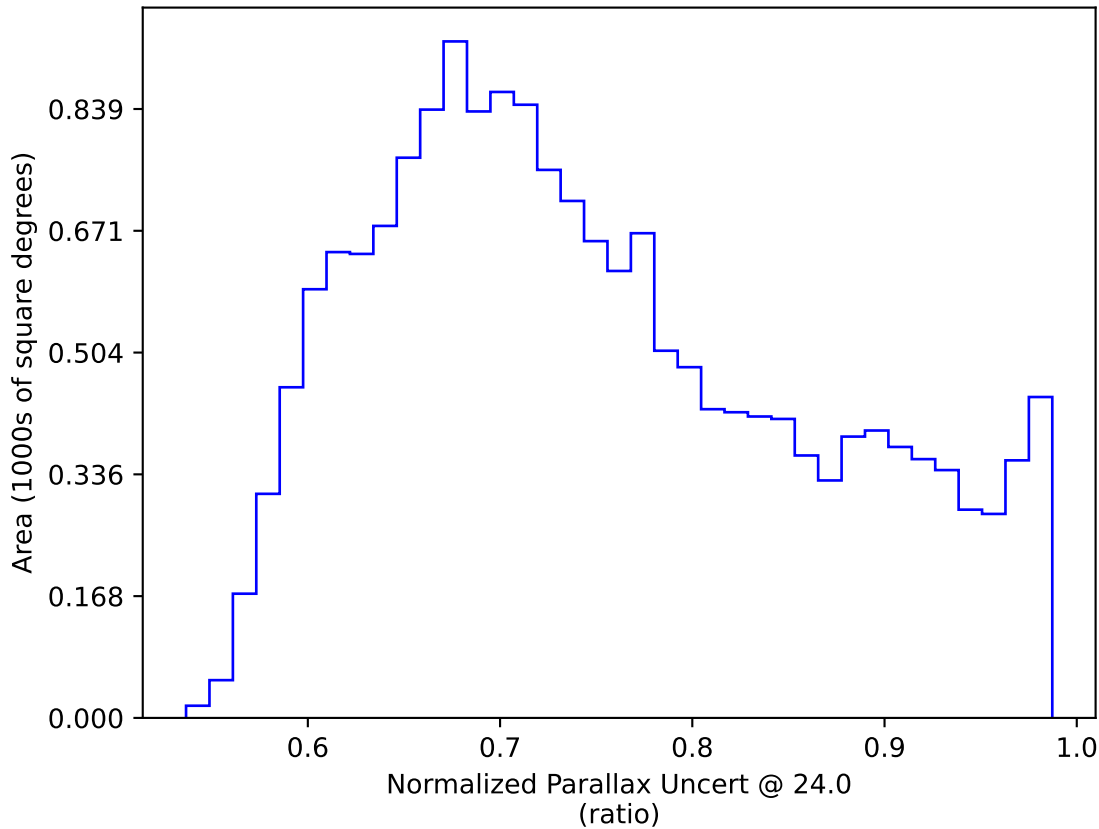
extra_ss_neo3_v3.4_10yrs WFD: Normalized Parallax Uncert @ 24.0
