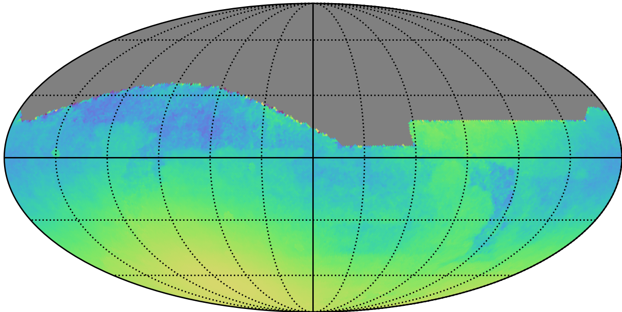
extra_ss_neo3_v3.4_10yrs All sky: Normalized Parallax Uncert @ 24.0
