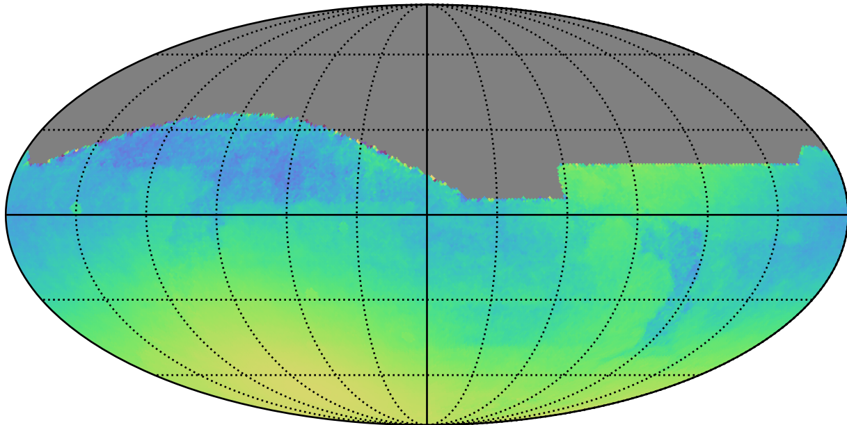
extra_ss_neo3_v3.4_10yrs All sky: Normalized Parallax Uncert @ 22.4
