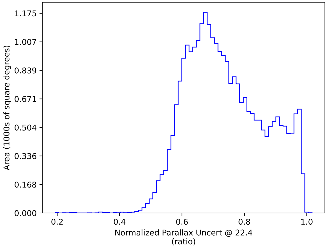
extra_ss_neo3_v3.4_10yrs All sky: Normalized Parallax Uncert @ 22.4
