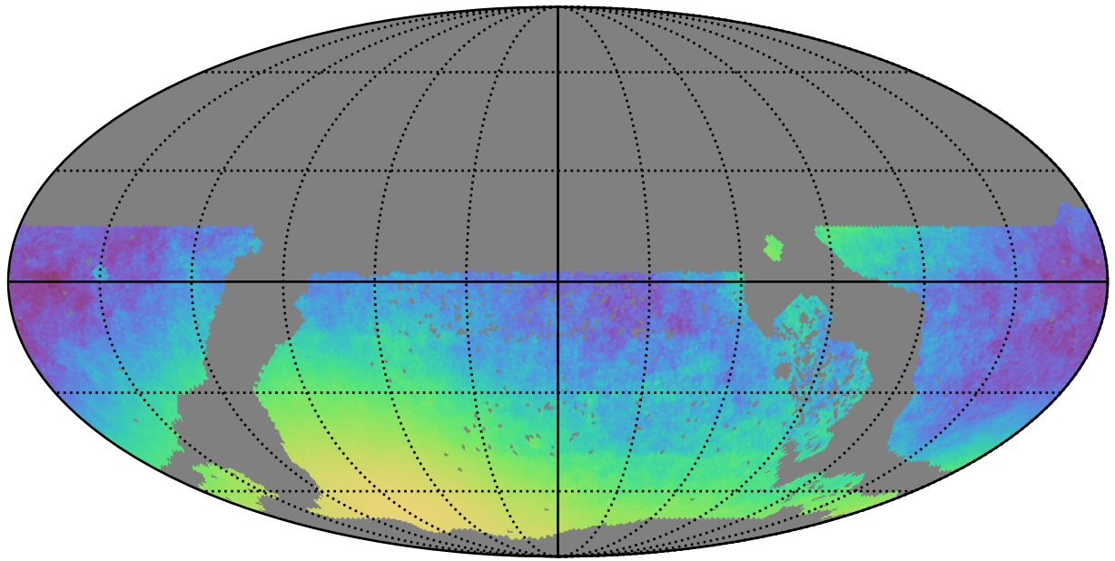
extra_ss_neo3_v3.4_10yrs WFD y band only: Normalized Parallax Uncert @ 21.3
