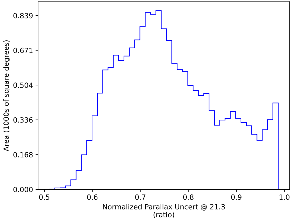
extra_ss_neo3_v3.4_10yrs WFD y band only: Normalized Parallax Uncert @ 21.3
