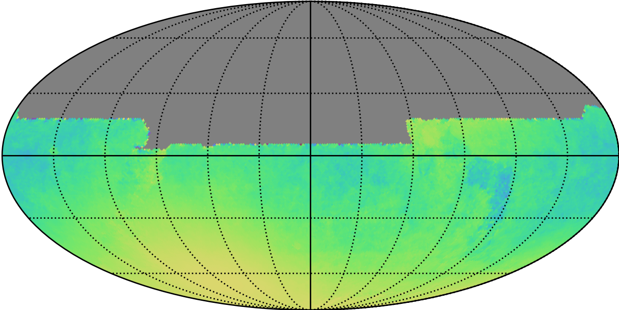
extra_ss_neo3_v3.4_10yrs All sky y band only: Normalized Parallax Uncert @ 21.3
