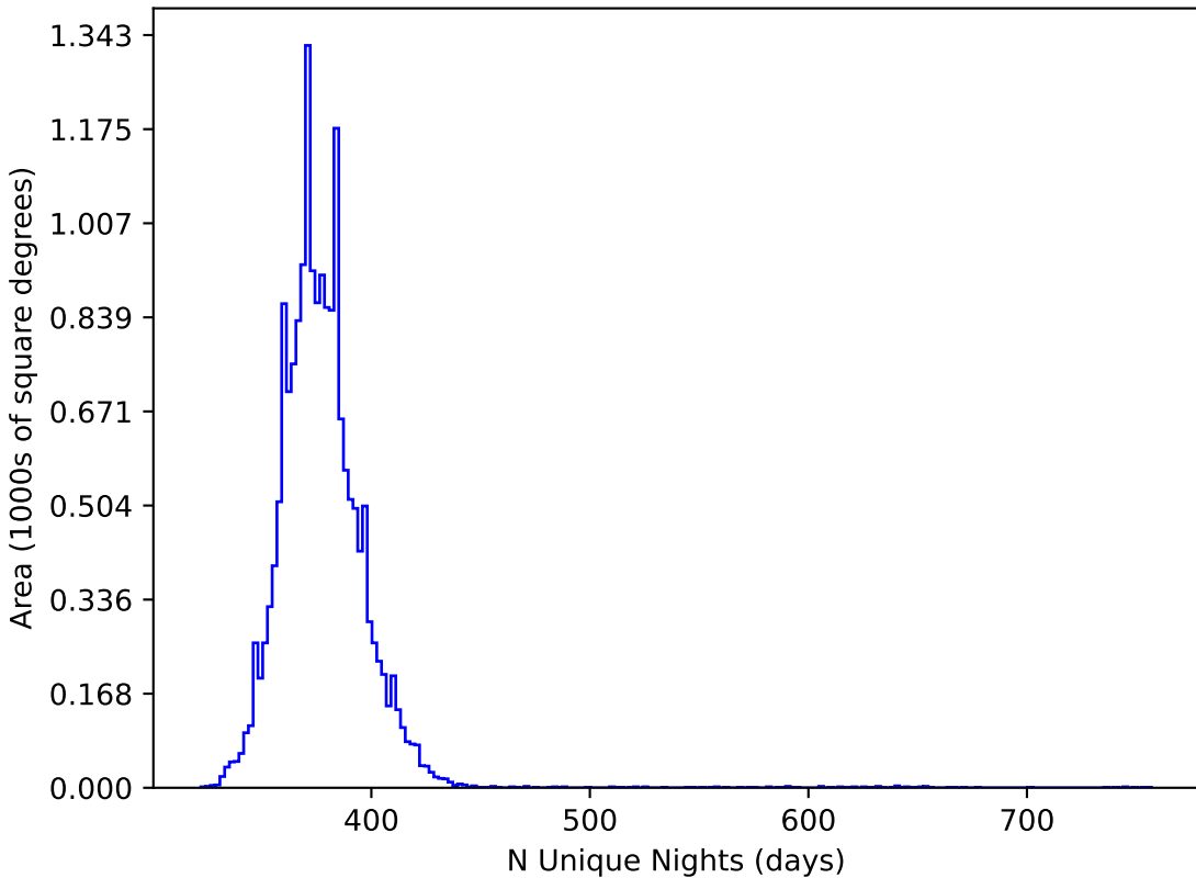
extra_ss_neo3_v3.4_10yrs WFD all bands: N Unique Nights
