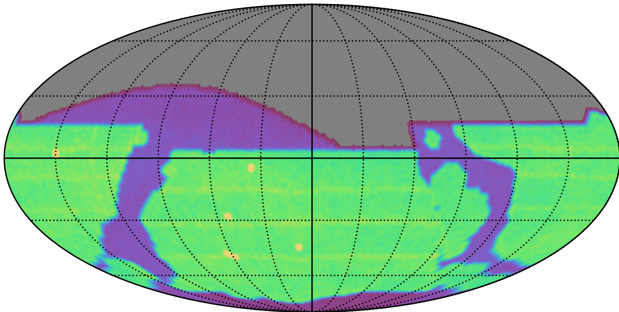
extra_ss_neo3_v3.4_10yrs All sky all bands: N Unique Nights
