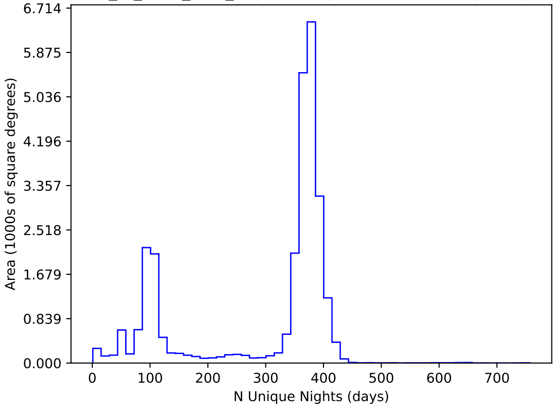
extra_ss_neo3_v3.4_10yrs All sky all bands: N Unique Nights
