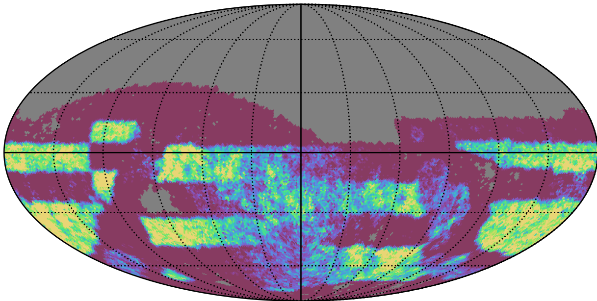
extra_ss_neo3_v3.4_10yrs Yr 3-4 z band: NVisits
