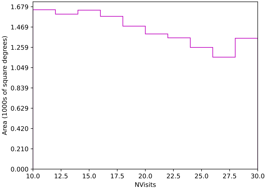
extra_ss_neo3_v3.4_10yrs Yr 3-4 z band: NVisits
