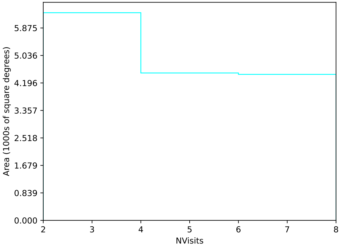
extra_ss_neo3_v3.4_10yrs Yr 3-4 u band: NVisits
