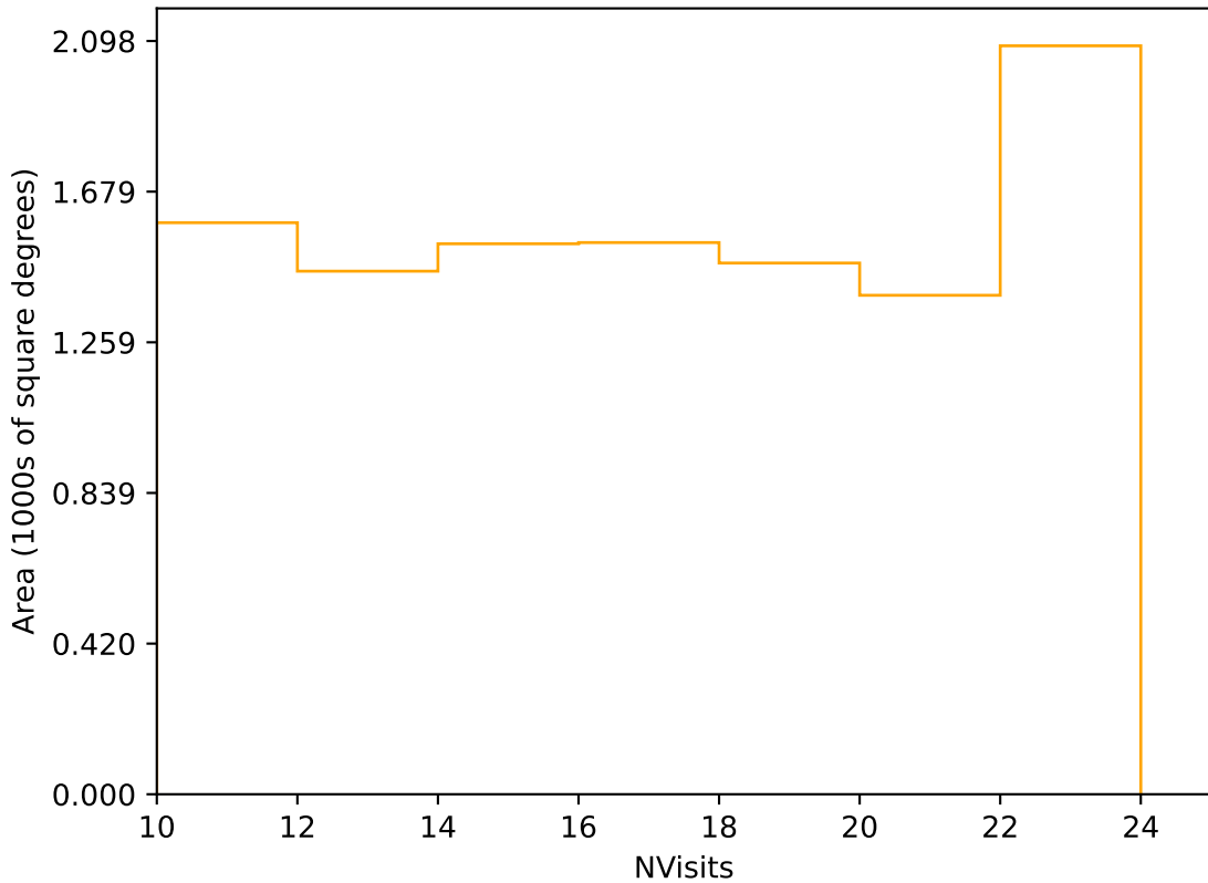
extra_ss_neo3_v3.4_10yrs Yr 3-4 r band: NVisits
