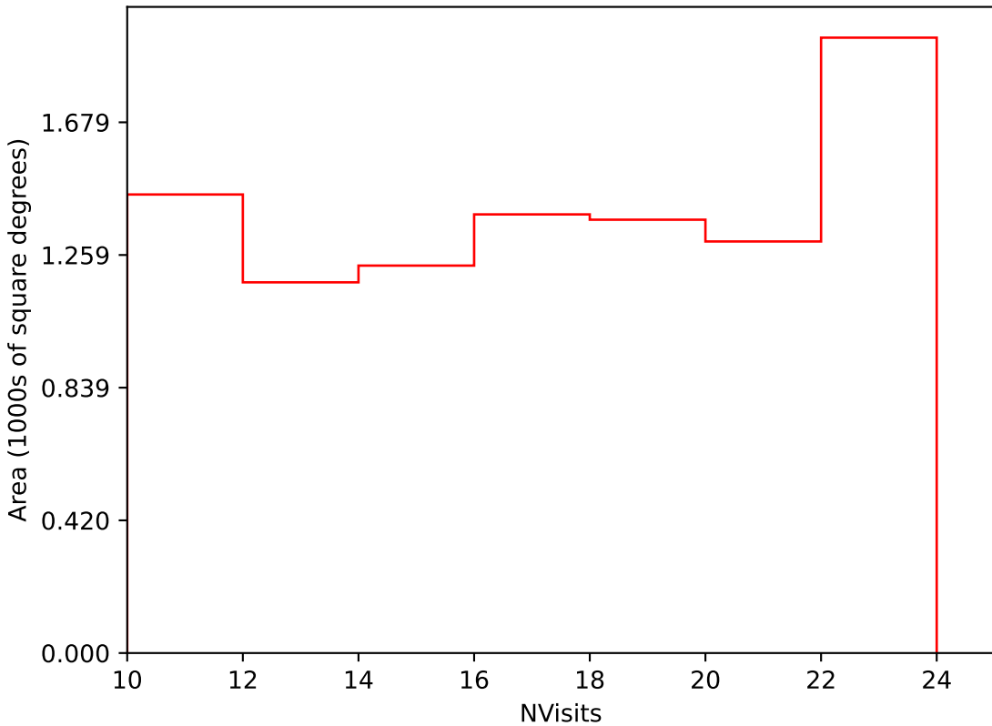
extra_ss_neo3_v3.4_10yrs Yr 3-4 i band: NVisits
