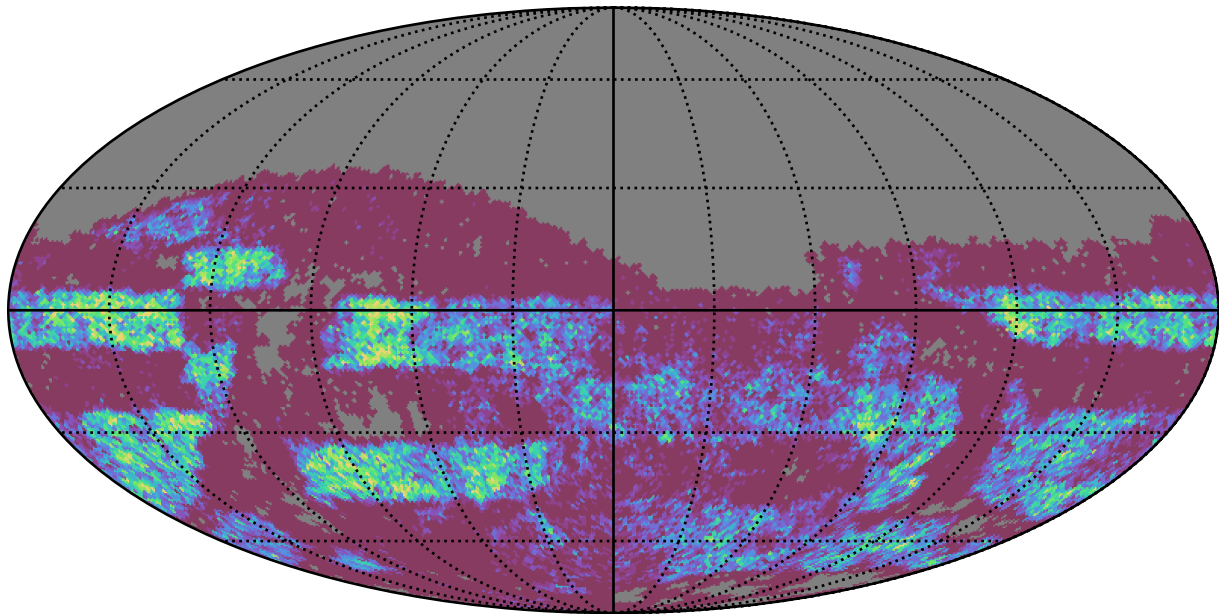
extra_ss_neo3_v3.4_10yrs Yr 3-4 g band: NVisits
