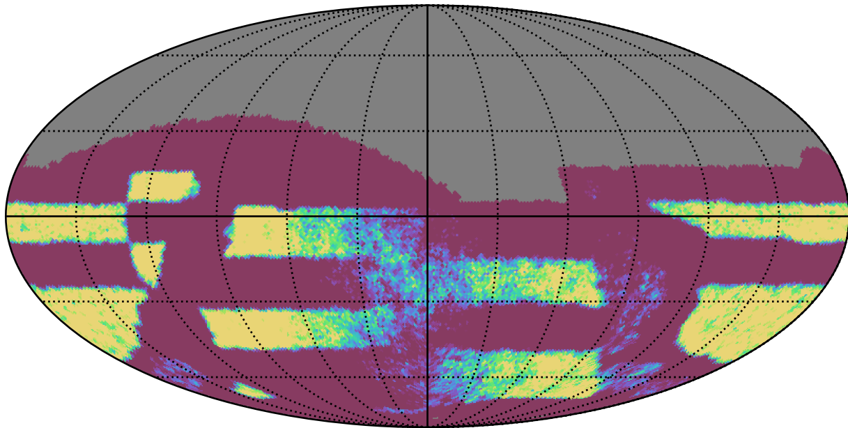
extra_ss_neo3_v3.4_10yrs Yr 3-4 all bands: NVisits
