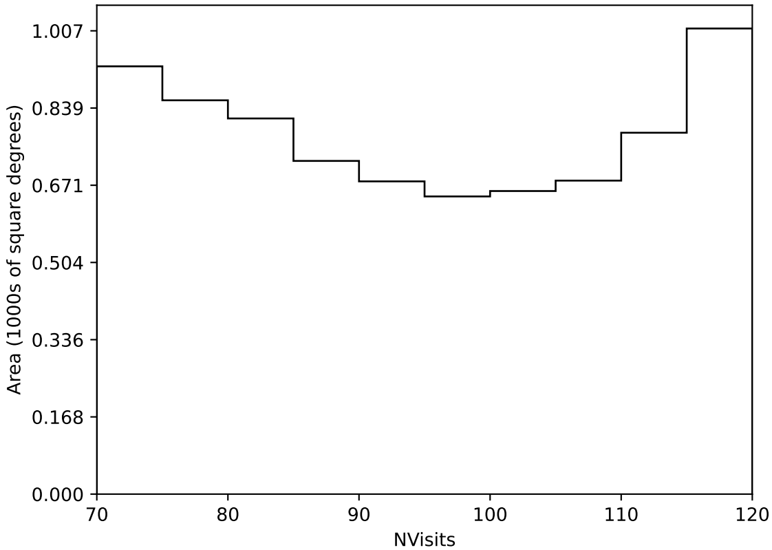
extra_ss_neo3_v3.4_10yrs Yr 3-4 all bands: NVisits
