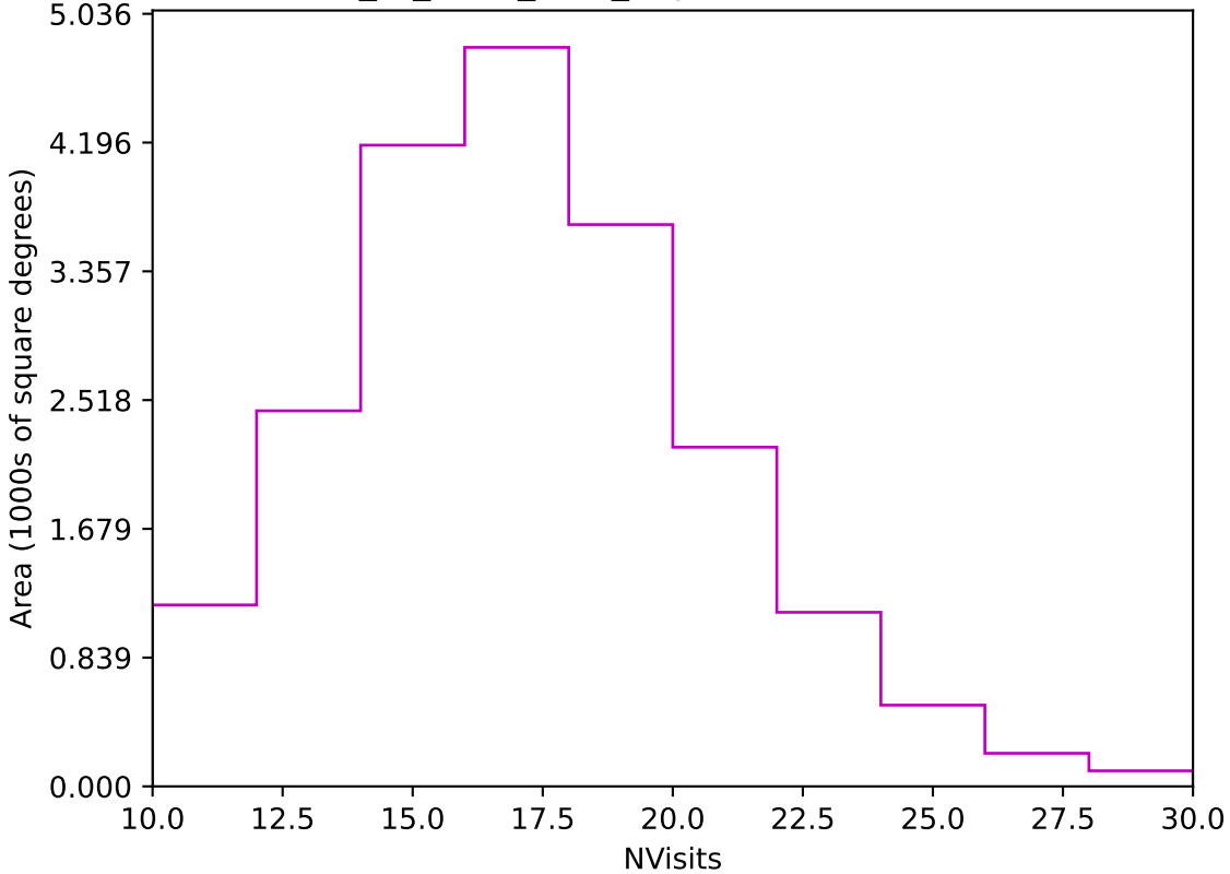
extra_ss_neo3_v3.4_10yrs Yr 1 z band: NVisits
