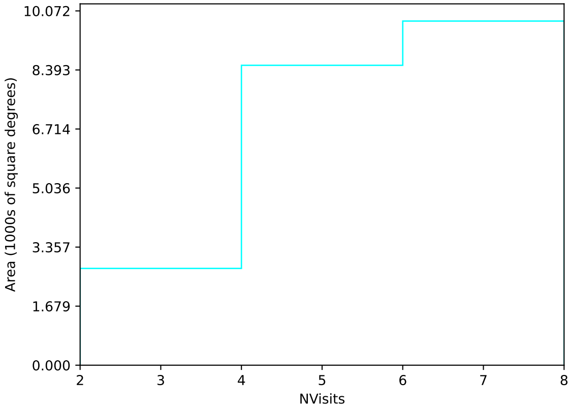
extra_ss_neo3_v3.4_10yrs Yr 1 u band: NVisits
