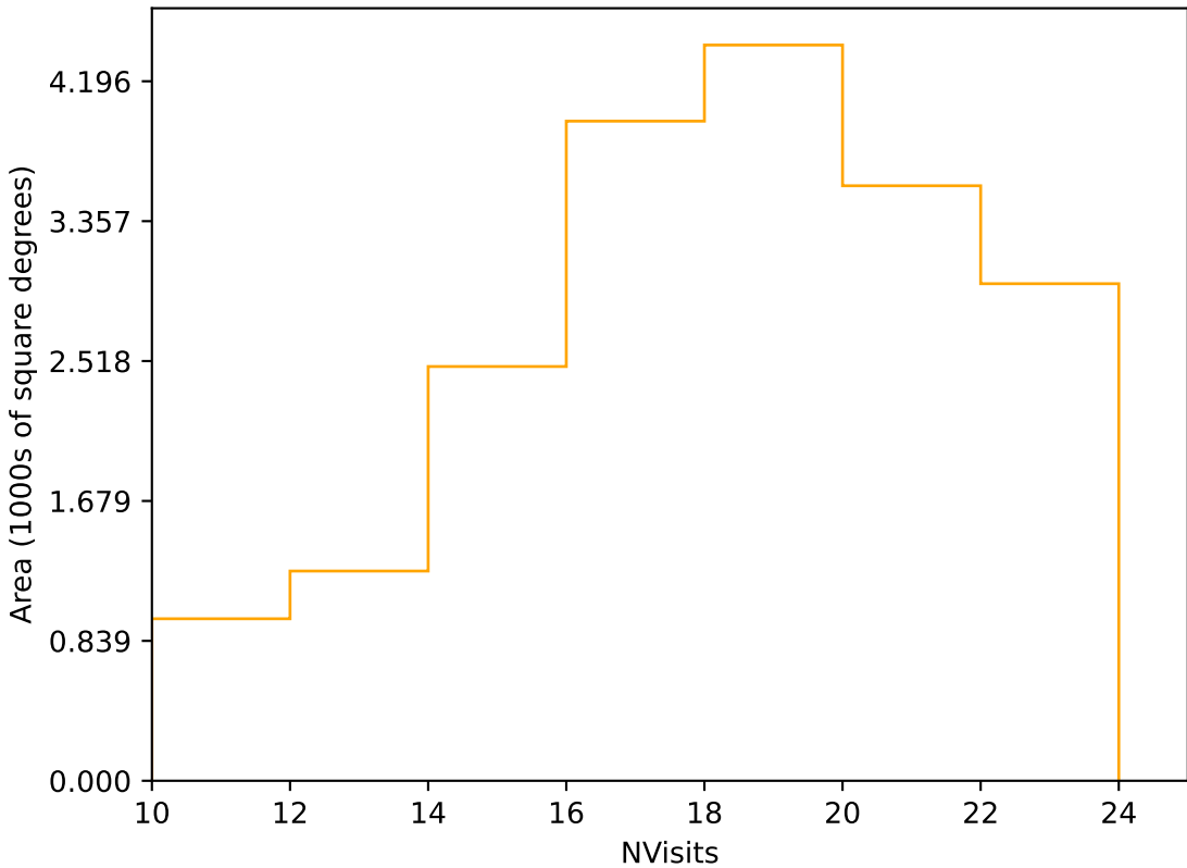
extra_ss_neo3_v3.4_10yrs Yr 1 r band: NVisits
