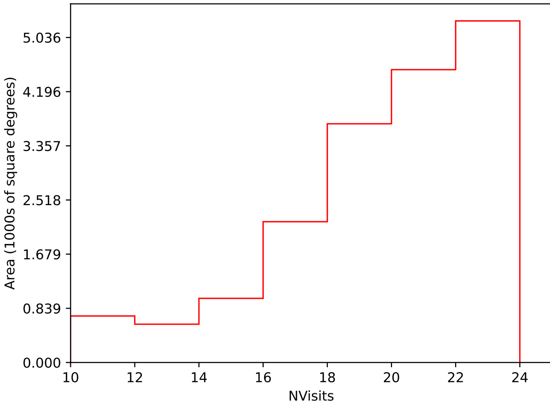
extra_ss_neo3_v3.4_10yrs Yr 1 i band: NVisits
