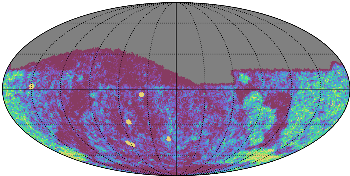
extra_ss_neo3_v3.4_10yrs Yr 1 g band: NVisits
