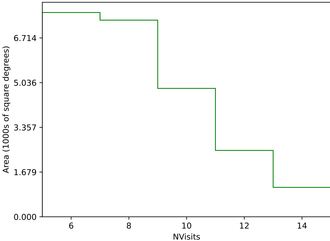
extra_ss_neo3_v3.4_10yrs Yr 1 g band: NVisits
