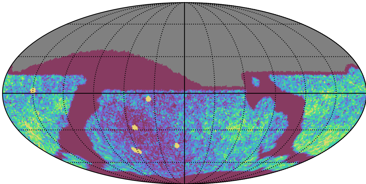
extra_ss_neo3_v3.4_10yrs Yr 1 all bands: NVisits
