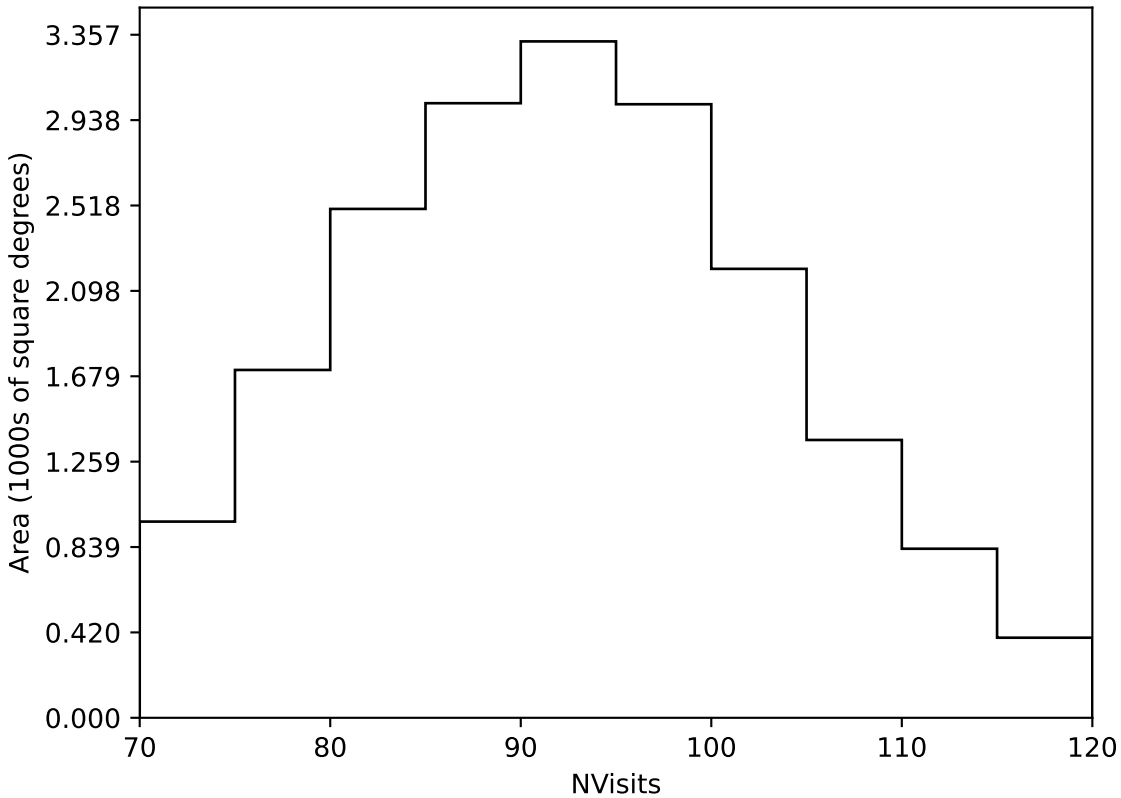
extra_ss_neo3_v3.4_10yrs Yr 1 all bands: NVisits
