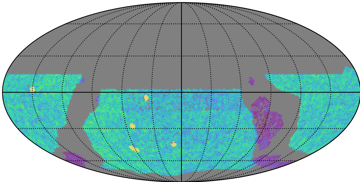
extra_ss_neo3_v3.4_10yrs WFD u band: NVisits
