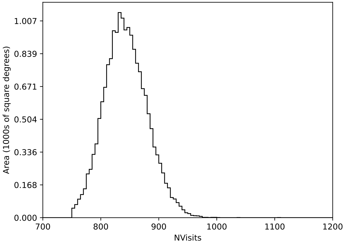
extra_ss_neo3_v3.4_10yrs WFD all bands: NVisits
