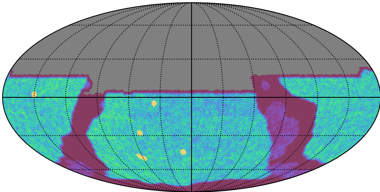
extra_ss_neo3_v3.4_10yrs All sky u band: NVisits
