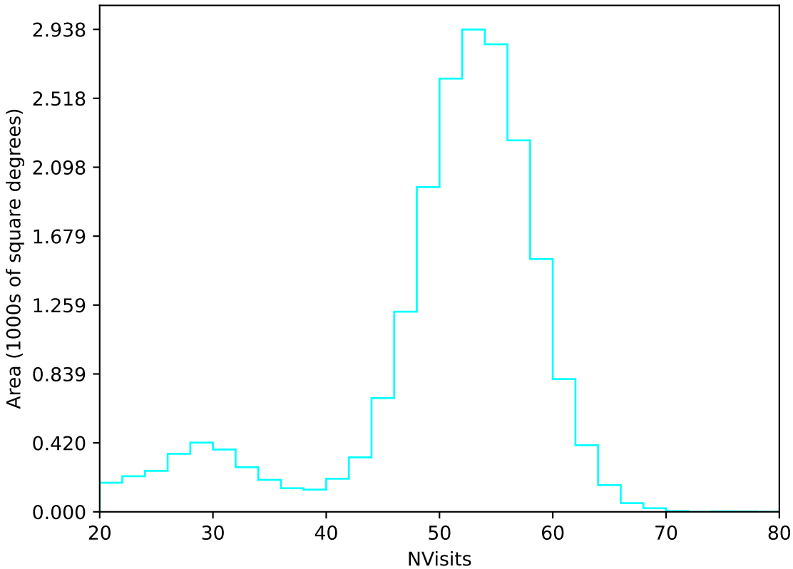
extra_ss_neo3_v3.4_10yrs All sky u band: NVisits
