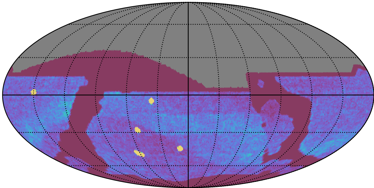
extra_ss_neo3_v3.4_10yrs All sky all bands: NVisits
