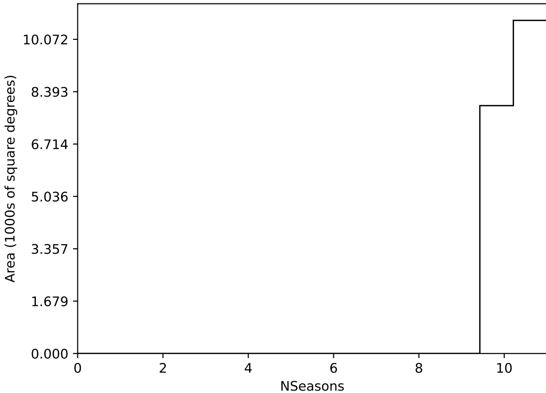
extra_ss_neo3_v3.4_10yrs WFD all bands: NSeasons
