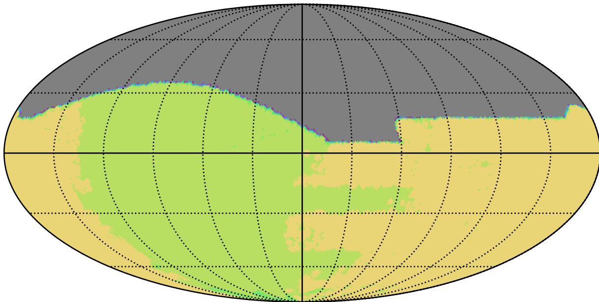
extra_ss_neo3_v3.4_10yrs All sky all bands: NSeasons
