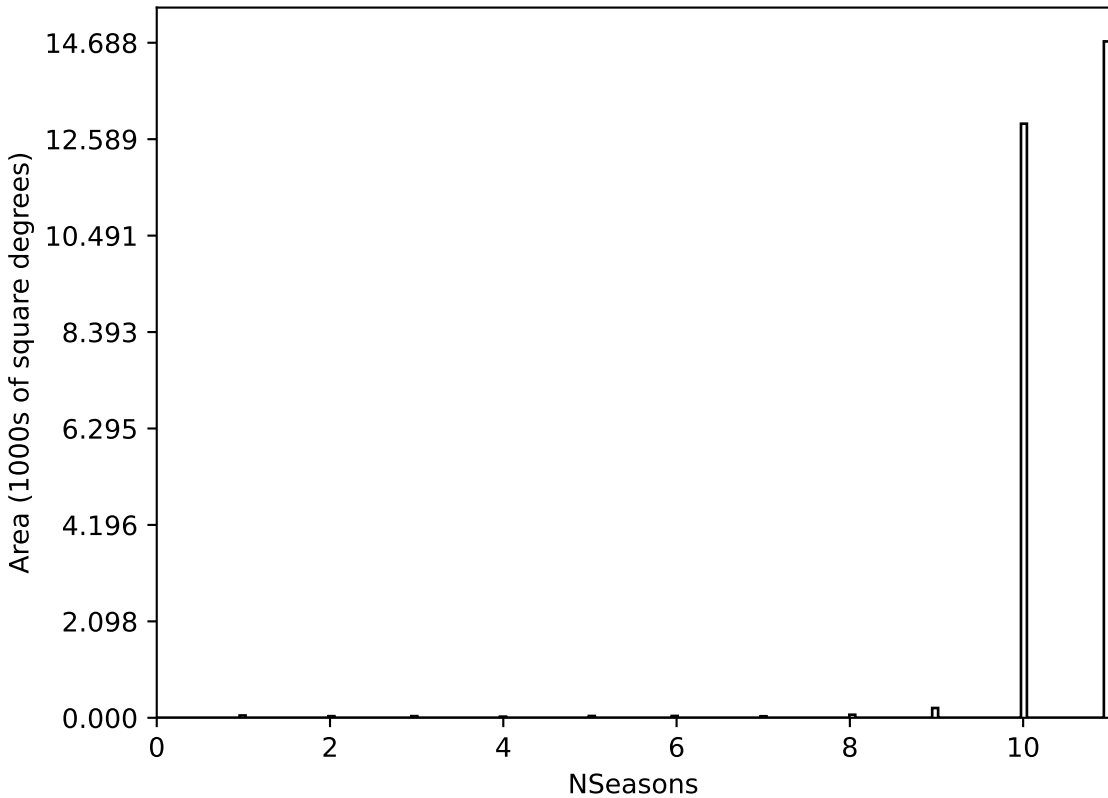
extra_ss_neo3_v3.4_10yrs All sky all bands: NSeasons
