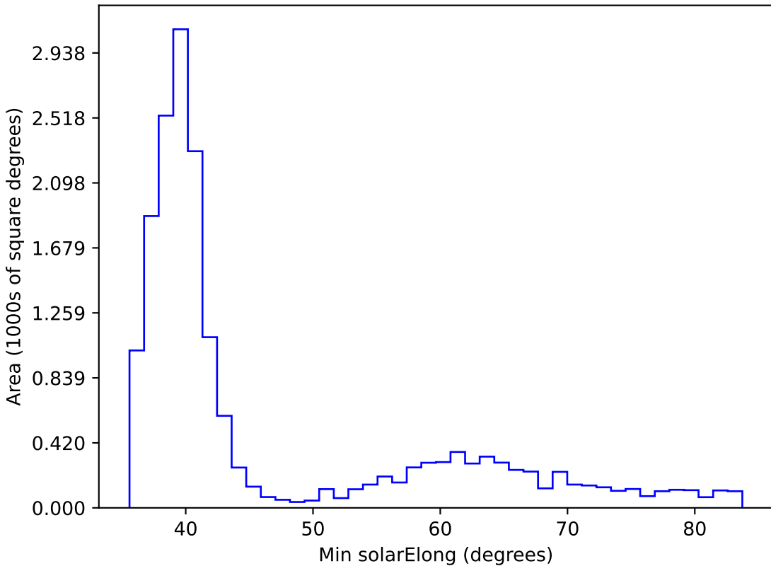
extra_ss_neo3_v3.4_10yrs WFD all bands: Min solarElong
