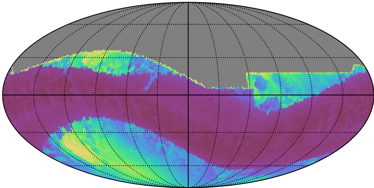
extra_ss_neo3_v3.4_10yrs All sky all bands: Min solarElong
