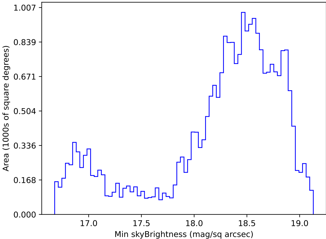
extra_ss_neo3_v3.4_10yrs Yr 1 z band: Min skyBrightness
