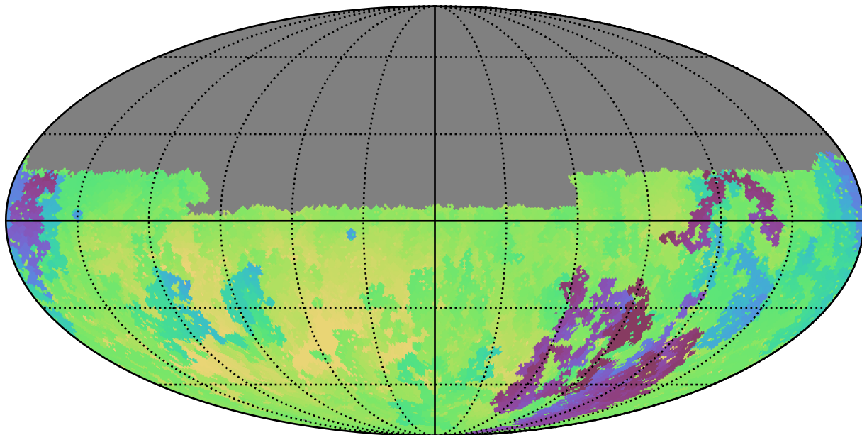
extra_ss_neo3_v3.4_10yrs Yr 1 u band: Min skyBrightness
