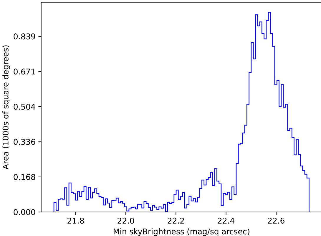
extra_ss_neo3_v3.4_10yrs Yr 1 u band: Min skyBrightness
