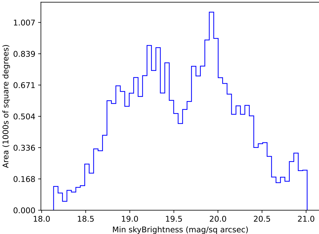
extra_ss_neo3_v3.4_10yrs Yr 1 r band: Min skyBrightness
