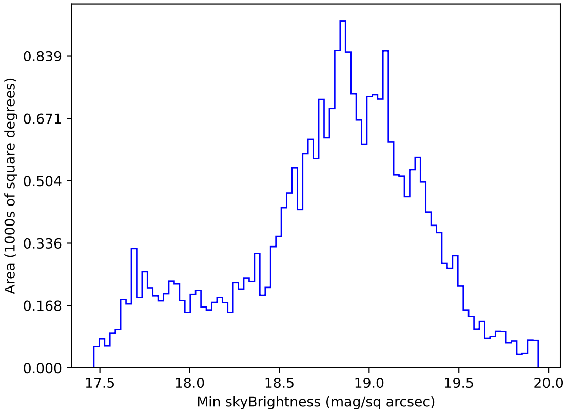
extra_ss_neo3_v3.4_10yrs Yr 1 i band: Min skyBrightness
