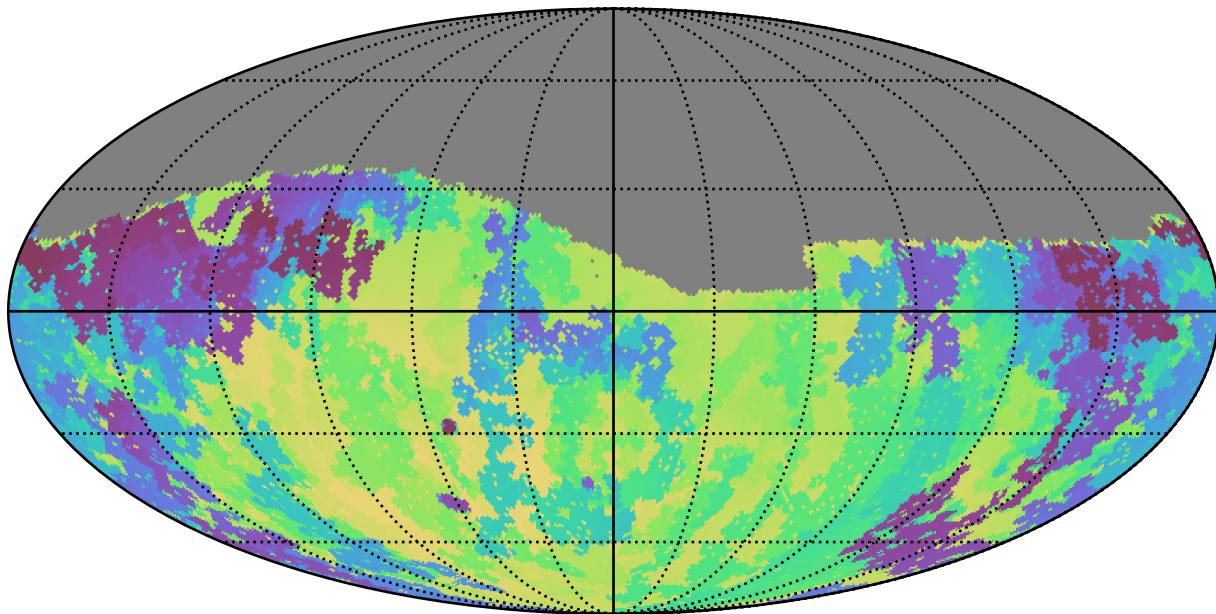
extra_ss_neo3_v3.4_10yrs Yr 1 g band: Min skyBrightness
