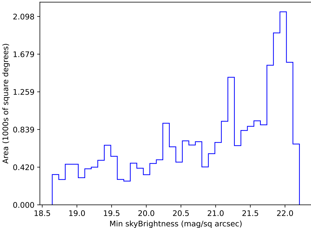
extra_ss_neo3_v3.4_10yrs Yr 1 g band: Min skyBrightness
