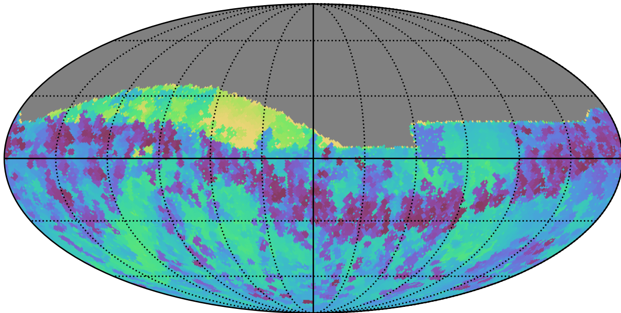
extra_ss_neo3_v3.4_10yrs Yr 1 all bands: Min skyBrightness
