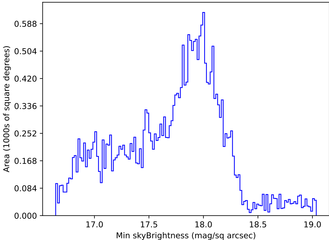
extra_ss_neo3_v3.4_10yrs Yr 1 all bands: Min skyBrightness
