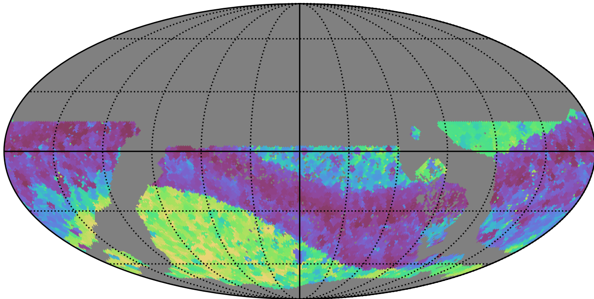
extra_ss_neo3_v3.4_10yrs WFD z band: Min skyBrightness
